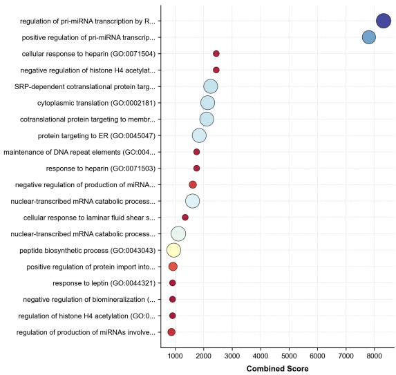
GO_BP enrichment (Top 20)
