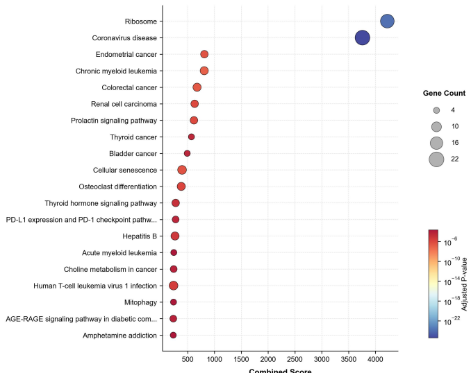
KEGG enrichment (Top 20)
